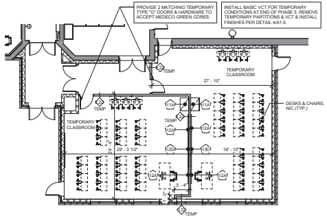
PHASE 3-5 TEMPORARY PARTITIONS 1/17-12/17
