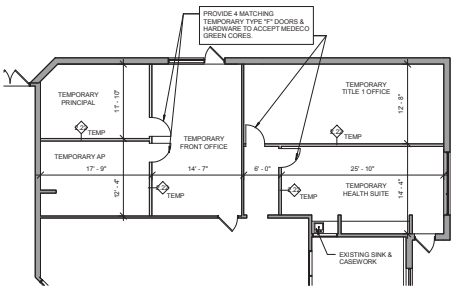
PHASE 1 TEMPORARY PARTITIONS 8/16-10/16
